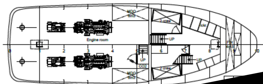
Lower deck - 1090 / OH 700 / OH
