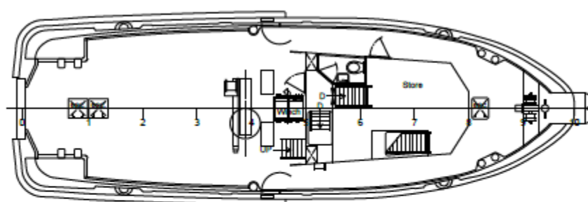
Main deck - 2700 / OH (Fr. 5)
